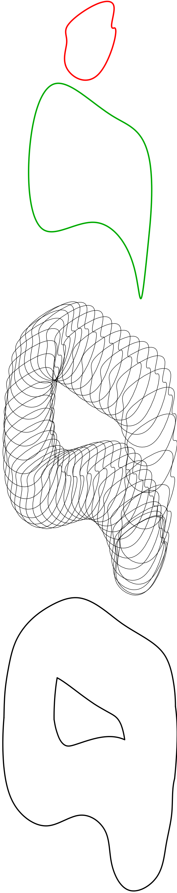
Figure 1: (a) The generator (b) The translation component of motion (c) Generator at a few time instants (d) The boundary of the swept volume.
