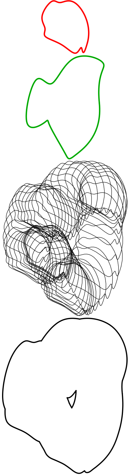
Figure 1: (a) The generator (b) The translation component of motion (c) Generator at a few time instants (d) The boundary of the swept volume.
