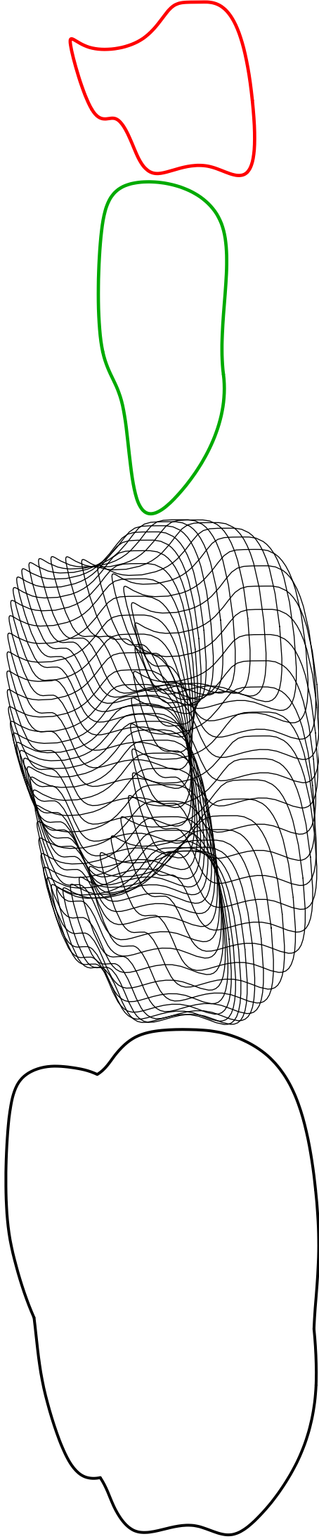
Figure 1: (a) The generator (b) The translation component of motion (c) Generator at a few time instants (d) The boundary of the swept volume.
