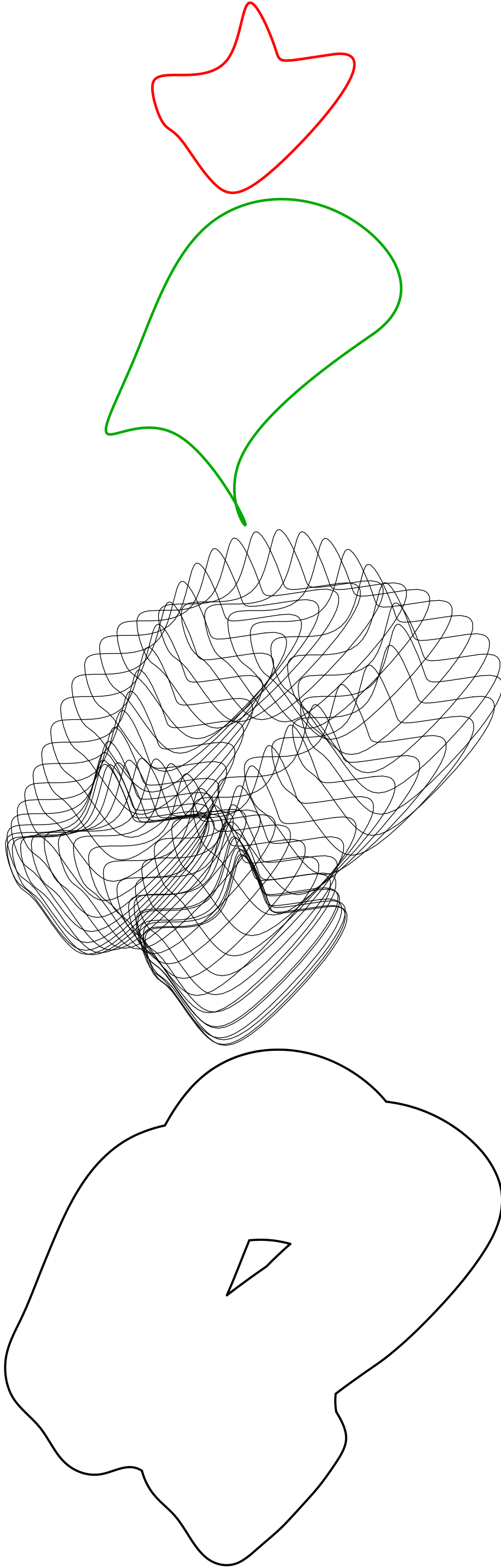
Figure 1: (a) The generator (b) The translation component of motion (c) Generator at a few time instants (d) The boundary of the swept volume.
