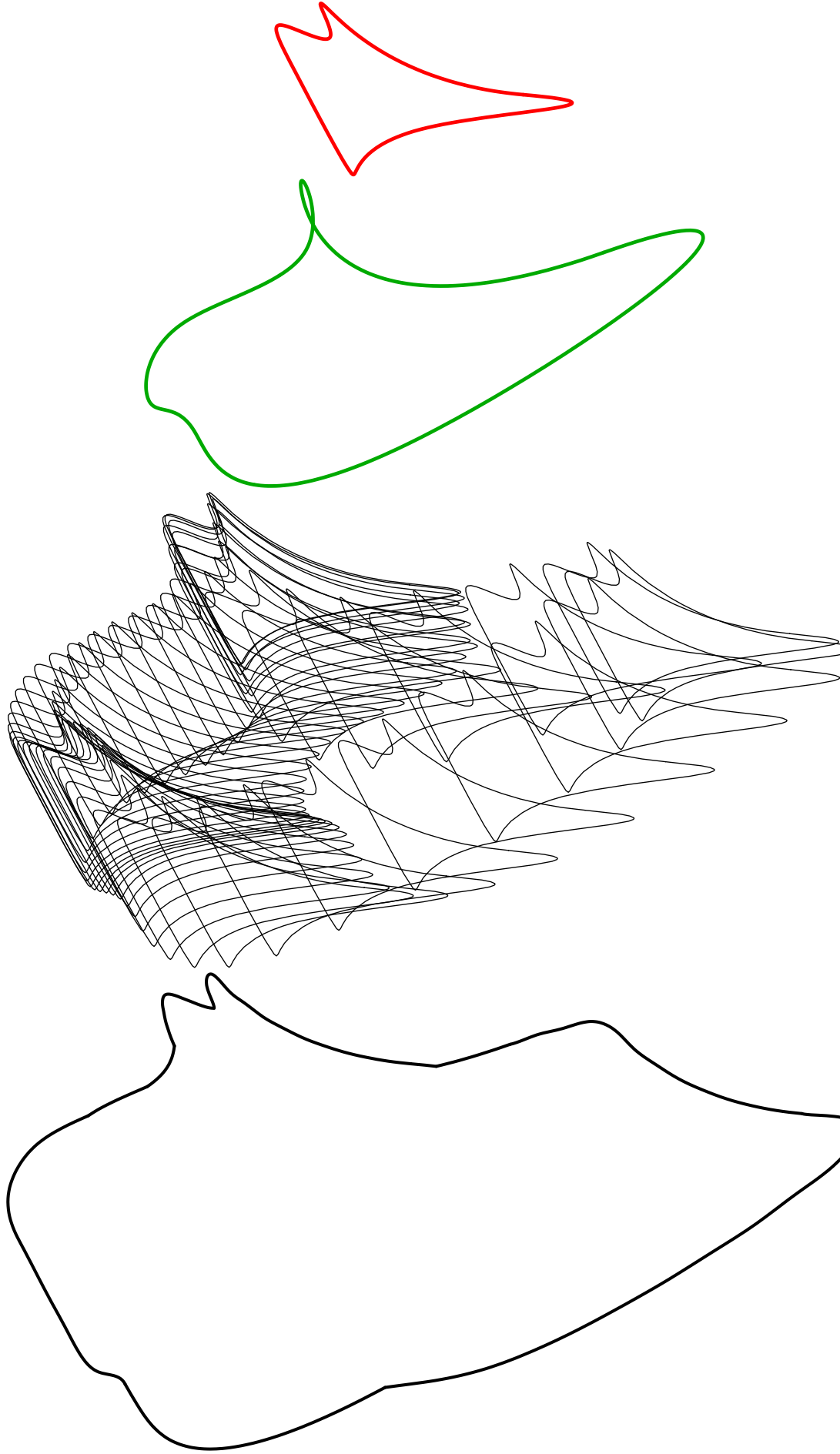
Figure 1: (a) The generator (b) The translation component of motion (c) Generator at a few time instants (d) The boundary of the swept volume.
