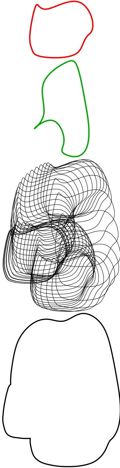
Figure 1: (a) The generator (b) The translation component of motion (c) Generator at a few time instants (d) The boundary of the swept volume.
