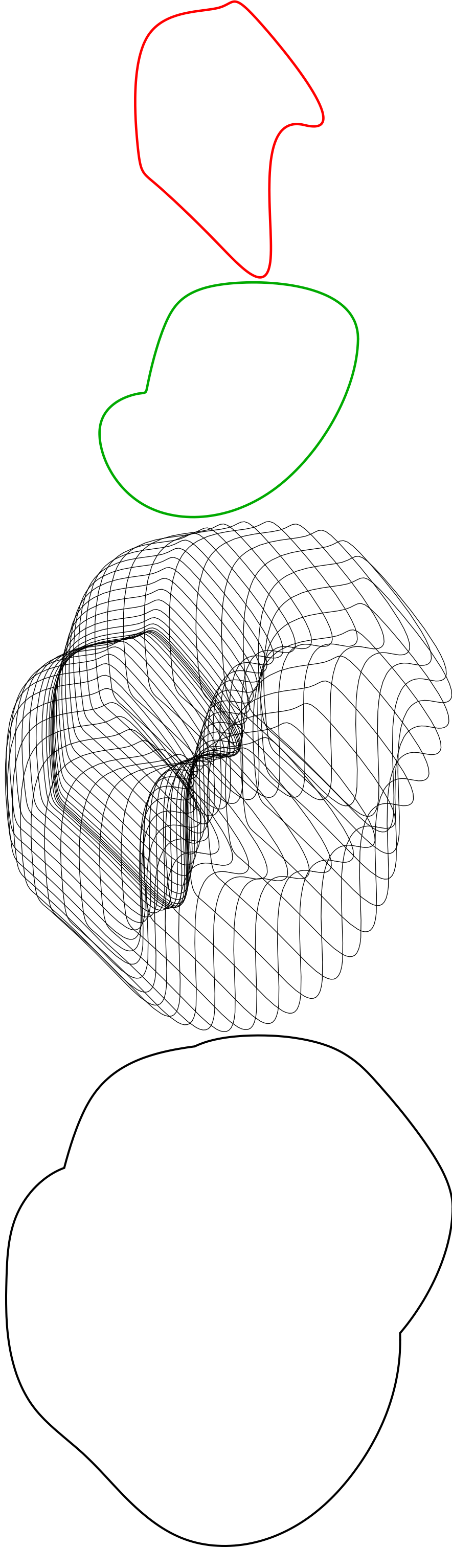
Figure 1: (a) The generator (b) The translation component of motion (c) Generator at a few time instants (d) The boundary of the swept volume.
