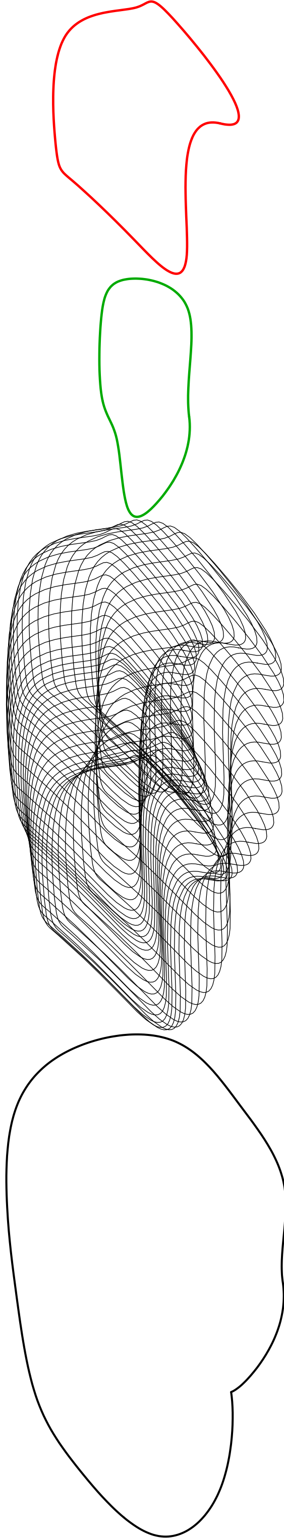
Figure 1: (a) The generator (b) The translation component of motion (c) Generator at a few time instants (d) The boundary of the swept volume.
