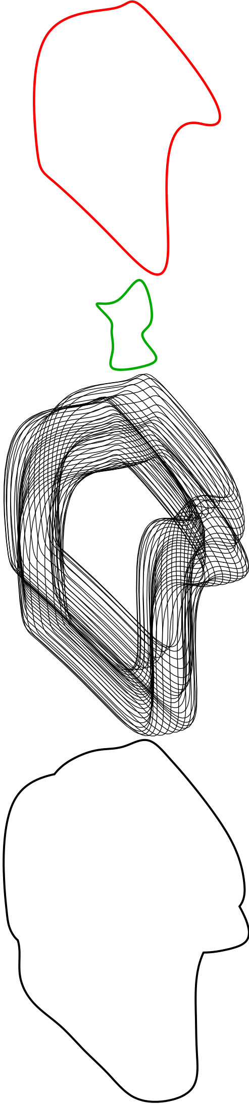
Figure 1: (a) The generator (b) The translation component of motion (c) Generator at a few time instants (d) The boundary of the swept volume.
