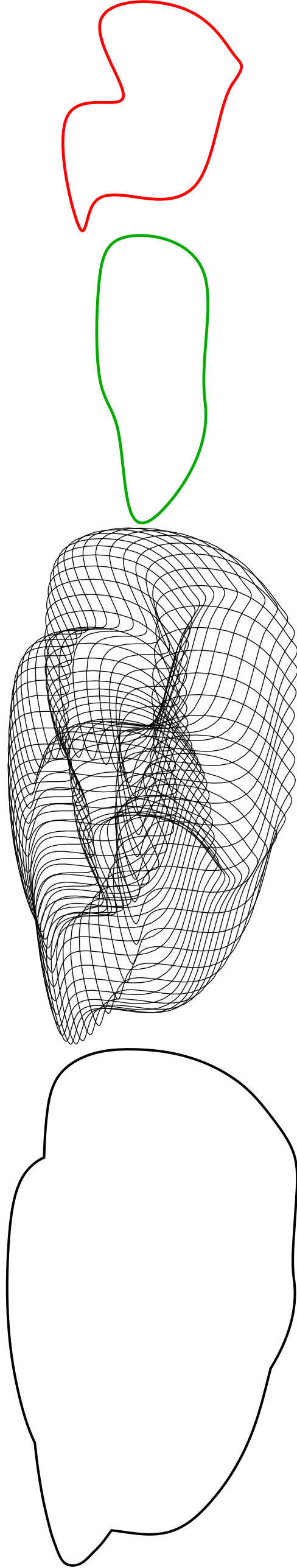
Figure 1: (a) The generator (b) The translation component of motion (c) Generator at a few time instants (d) The boundary of the swept volume.
