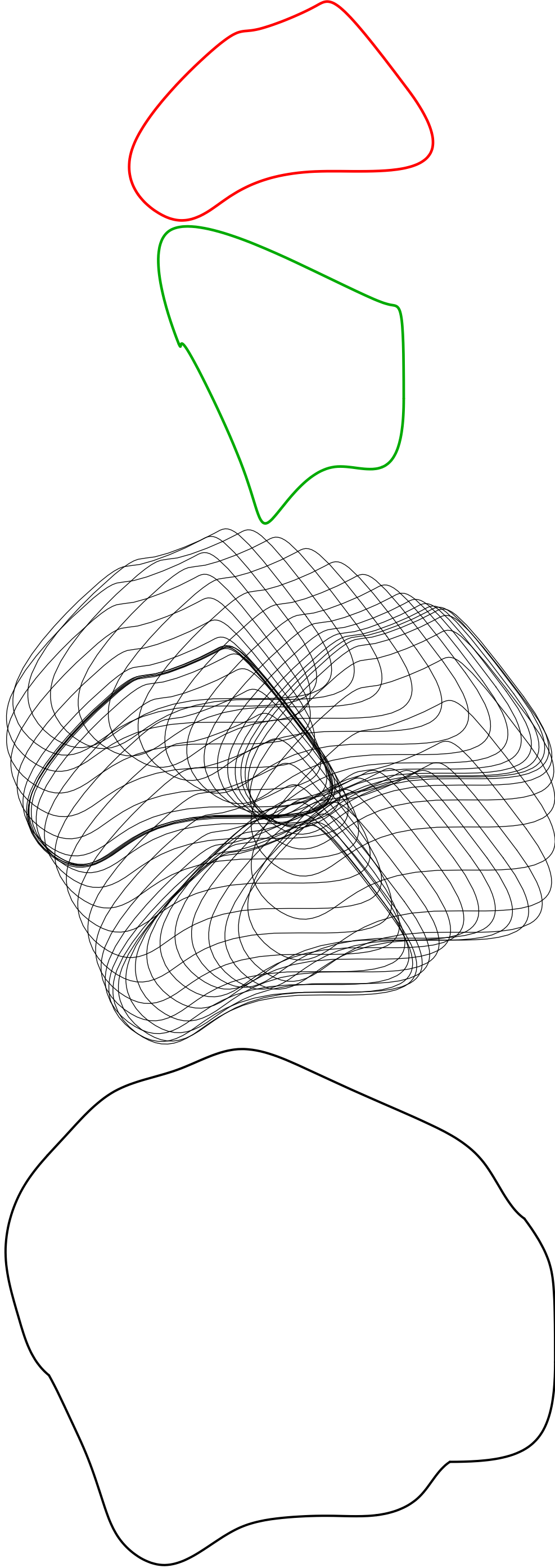
Figure 1: (a) The generator (b) The translation component of motion (c) Generator at a few time instants (d) The boundary of the swept volume.
