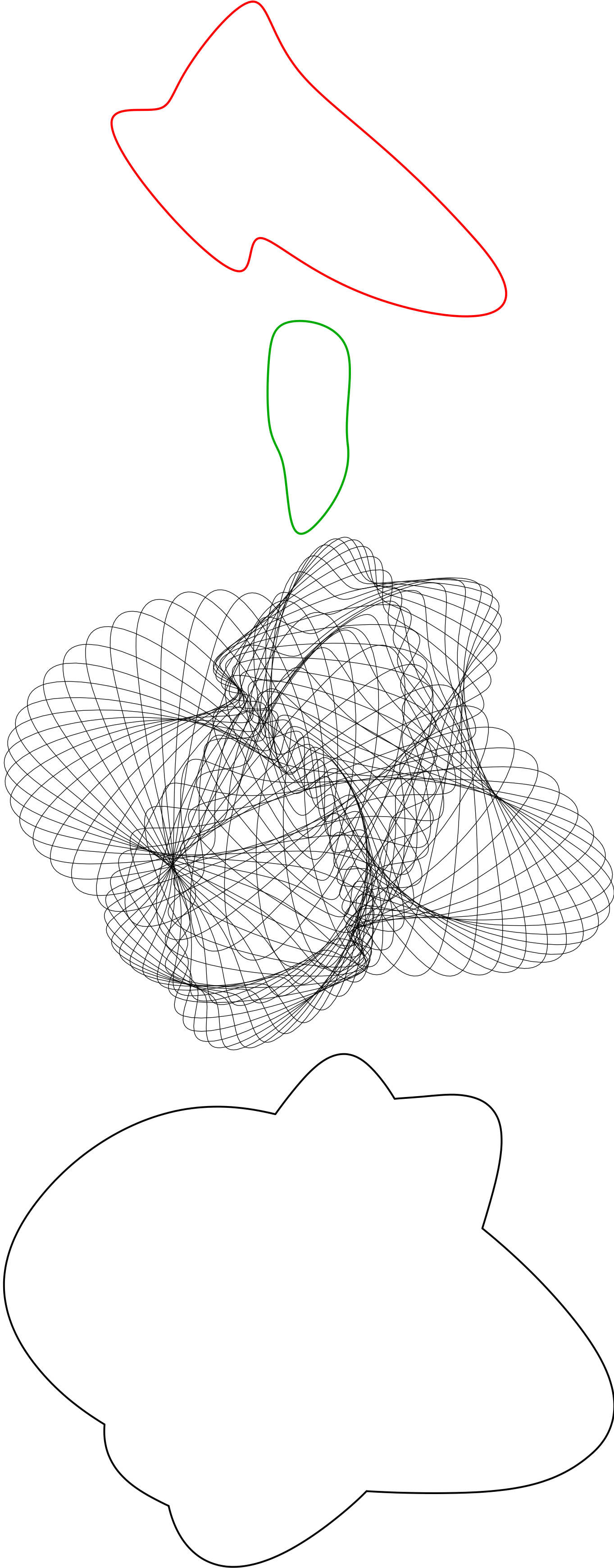
Figure 1: (a) The generator (b) The translation component of motion (c) Generator at a few time instants (d) The boundary of the swept volume.
