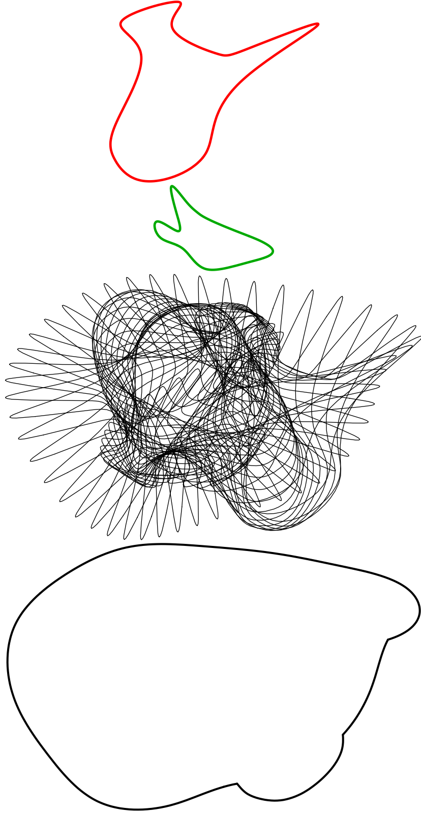
Figure 1: (a) The generator (b) The translation component of motion (c) Generator at a few time instants (d) The boundary of the swept volume.
