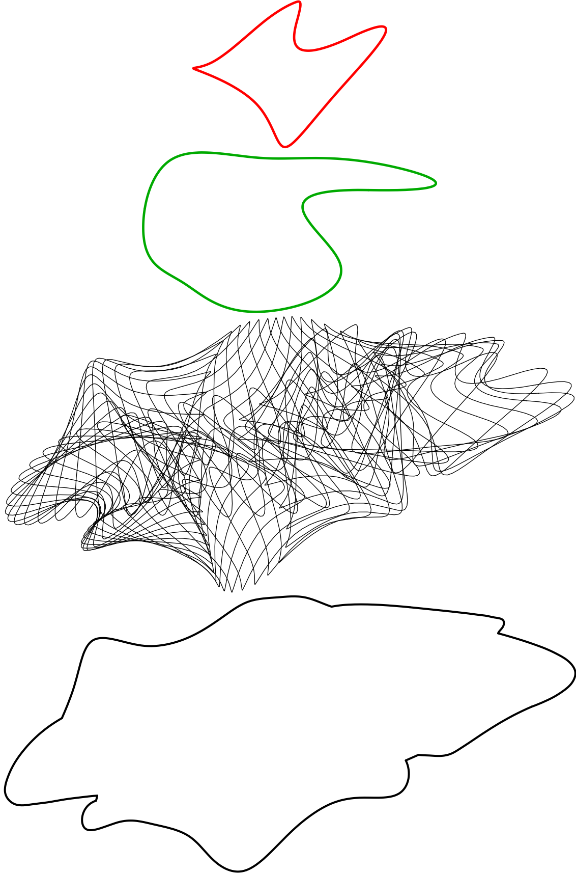
Figure 1: (a) The generator (b) The translation component of motion (c) Generator at a few time instants (d) The boundary of the swept volume.
