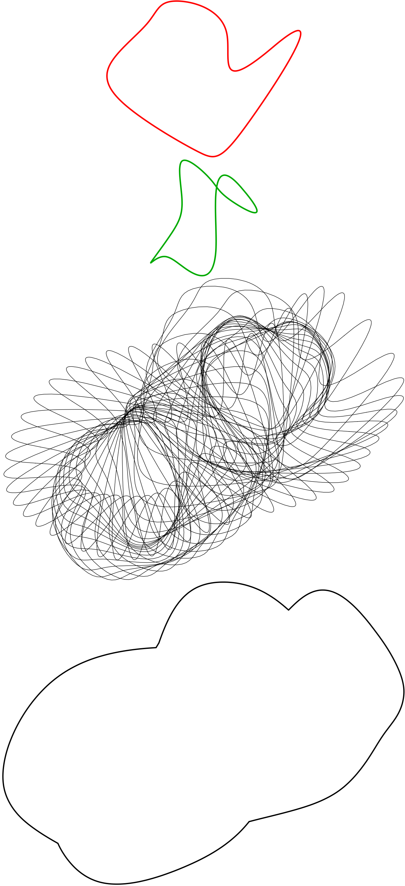
Figure 1: (a) The generator (b) The translation component of motion (c) Generator at a few time instants (d) The boundary of the swept volume.
