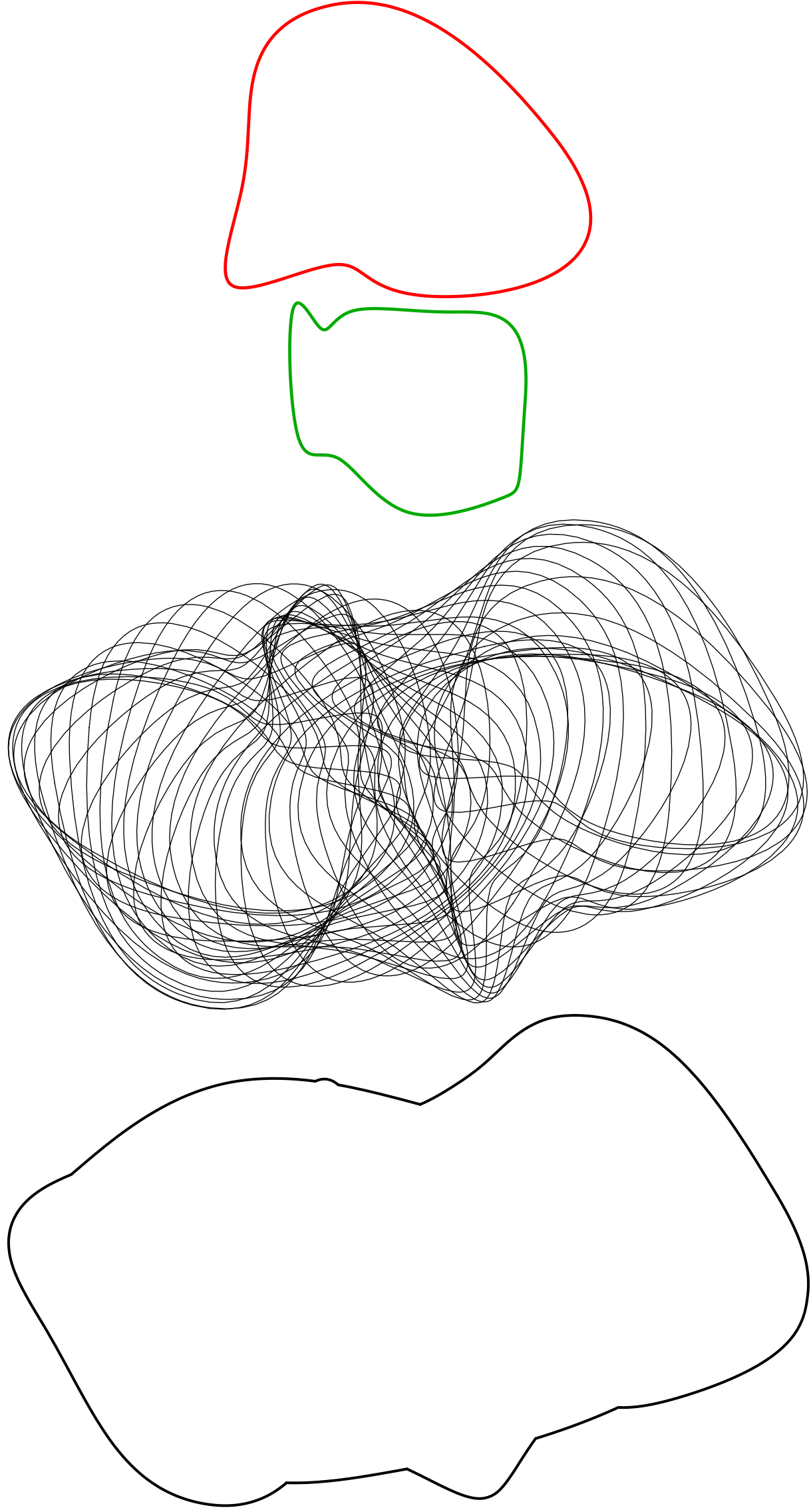
Figure 1: (a) The generator (b) The translation component of motion (c) Generator at a few time instants (d) The boundary of the swept volume.
