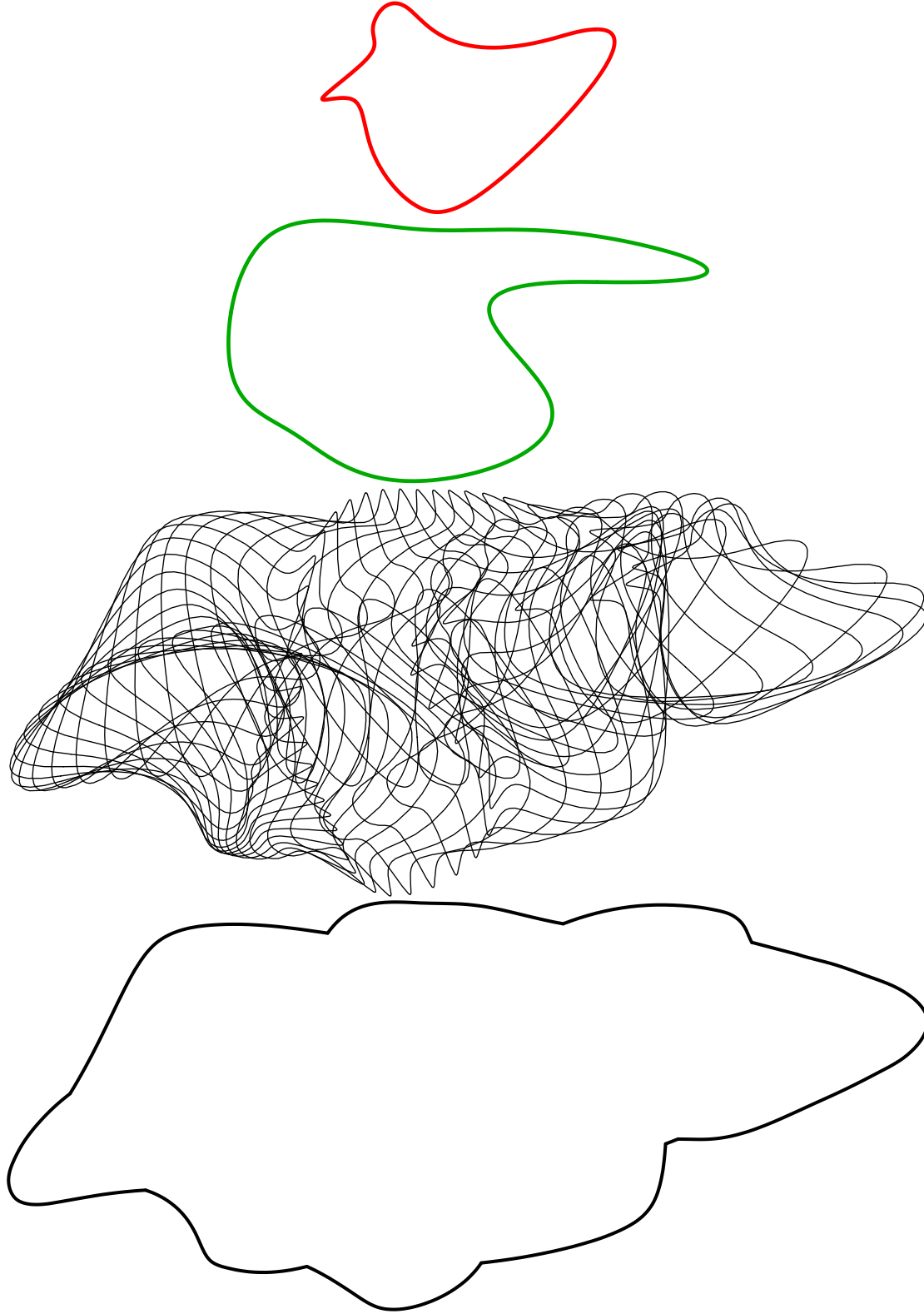
Figure 1: (a) The generator (b) The translation component of motion (c) Generator at a few time instants (d) The boundary of the swept volume.
