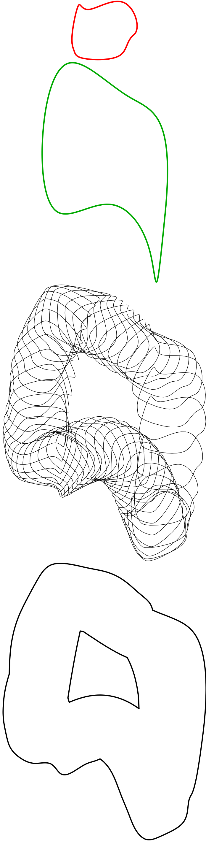
Figure 1: (a) The generator (b) The translation component of motion (c) Generator at a few time instants (d) The boundary of the swept volume.
