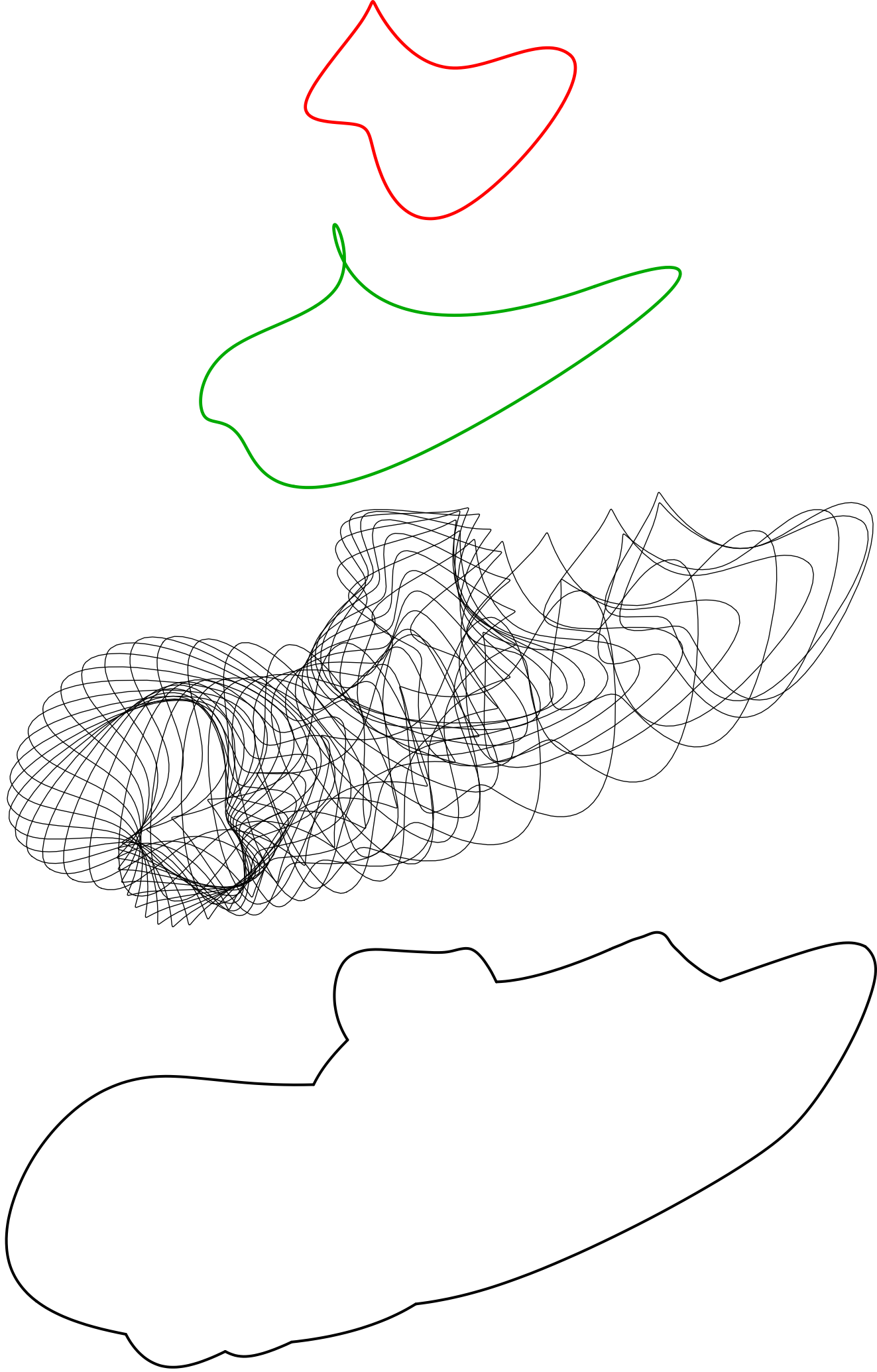
Figure 1: (a) The generator (b) The translation component of motion (c) Generator at a few time instants (d) The boundary of the swept volume.
