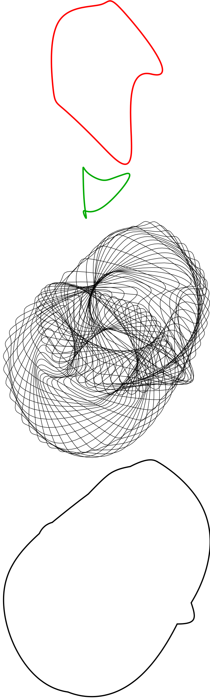
Figure 1: (a) The generator (b) The translation component of motion (c) Generator at a few time instants (d) The boundary of the swept volume.
