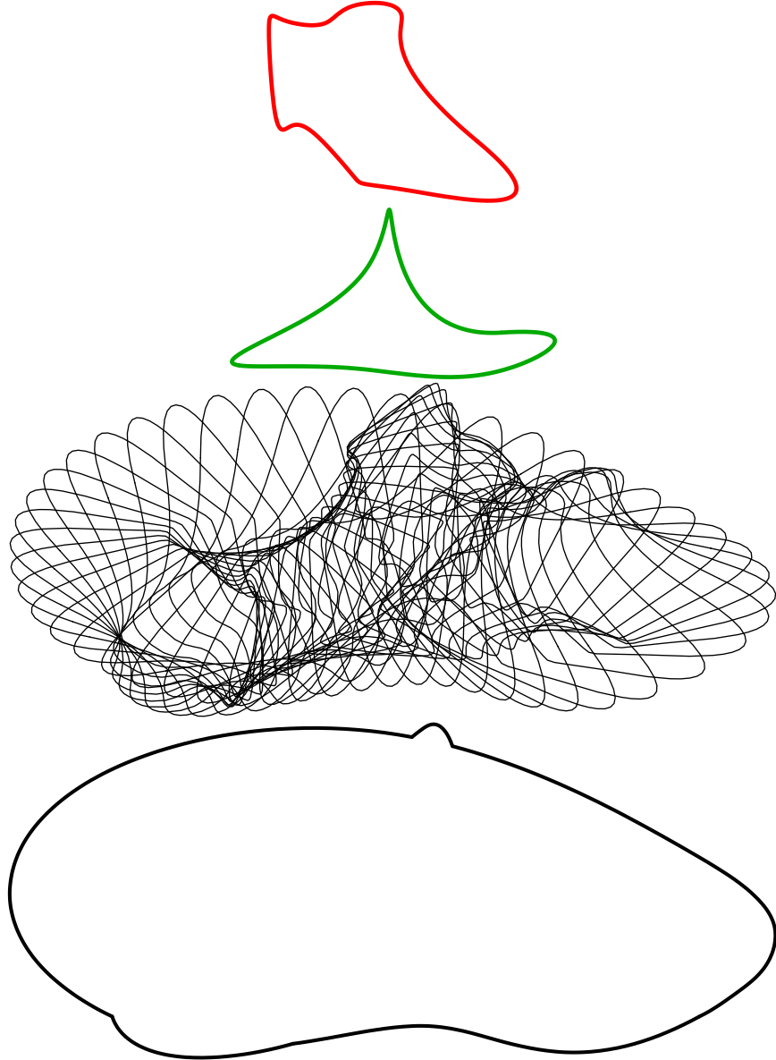
Figure 1: (a) The generator (b) The translation component of motion (c) Generator at a few time instants (d) The boundary of the swept volume.
